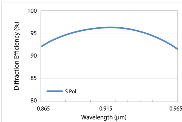
Typical absolute diffraction efficiency at AOI 57.9° *
