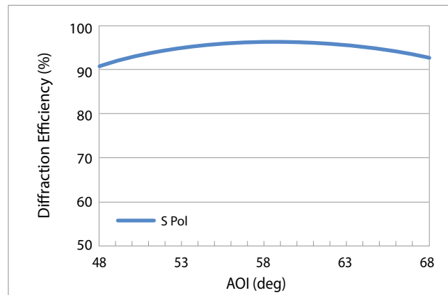
Diffraction efficiency at 915 nm as a function of AOI *
