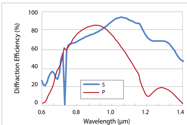
Typical absolute diffraction efficiency at AOI 58° *
