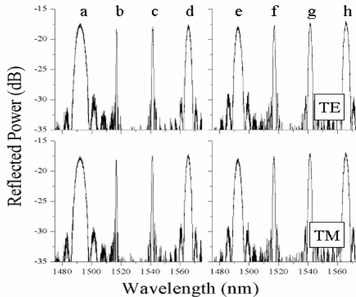
Fig. 3. Reflection spectra of two channel waveguides (left and right) each containing four separate gratings. Top and bottom rows show different input polarizations. Each individual grating is written with identical contour sets adjusted to specific field reflectivity and grating lengths are adjusted to provide nearly uniform net reflectivity (see text).
