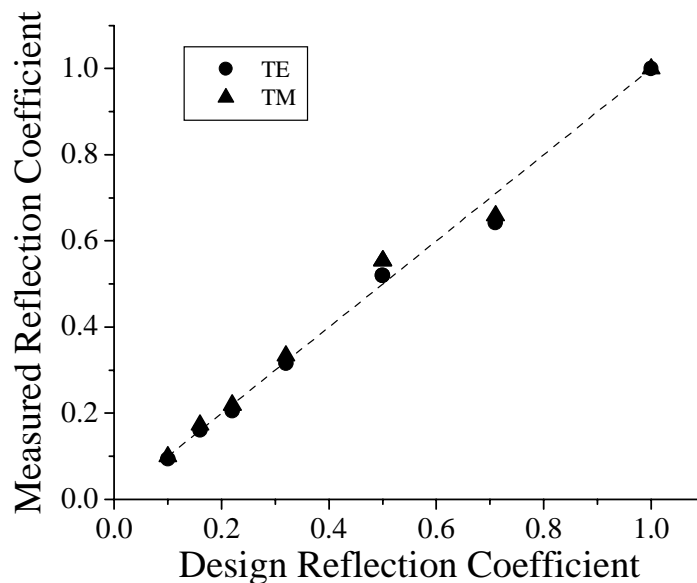
Fig. 4. Plot of measured amplitude reflection coefficient versus design reflection coefficient for the gratings of Table 1.
