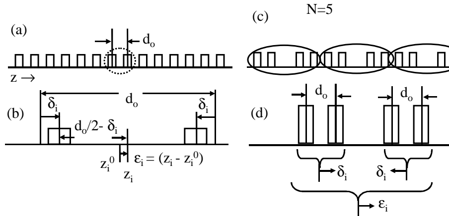
Fig. 2. Basic concept of correlated-contour amplitude and phase control. (a) Uniform grating. (b) Blow-up of two adjacent grating contours with common and differential position shifts. (c) Five-contour subgroups with center contour deletion to provide room for centerwise displacement of outer contours. (d) Common mode and differential displacements of contour set elements ( N=5 ) used to adjust phase and amplitude, respectively.
