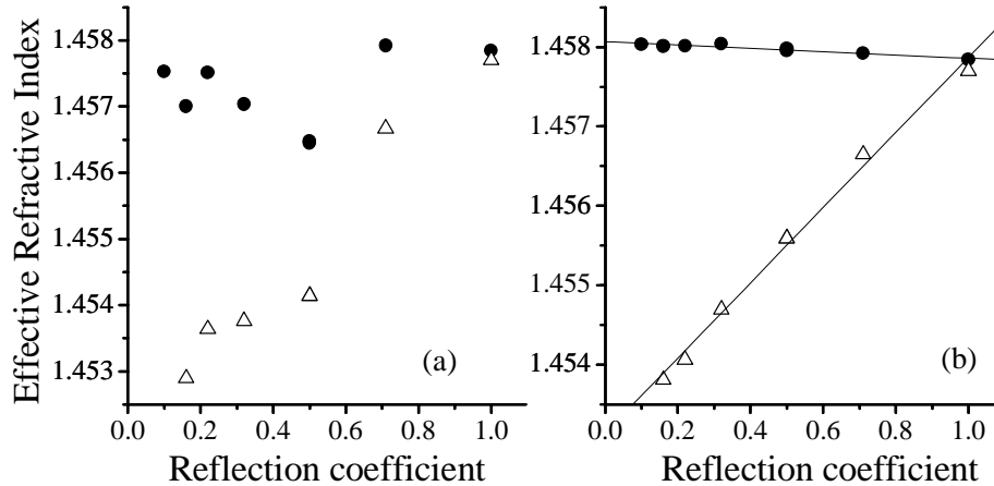
Fig. 5. (a) Measured effective refractive index as a function of amplitude reflection coefficient for correlated-line-set gratings (solid circles) and a reference grating set (open triangles) whose reflectivity is controlled via the partial scribe method of Ref. 8. (b) Effective refractive index of the two grating sets after extracting intrinsic wavelength dependence.
